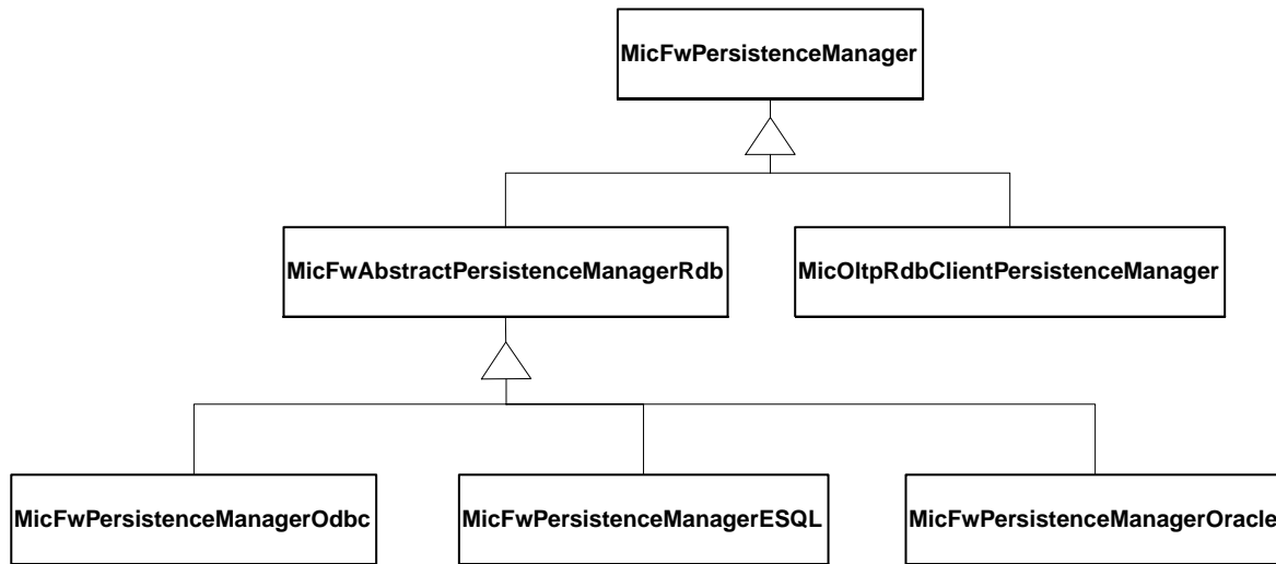
Figure 4: Persistence Manager Hierarchy
