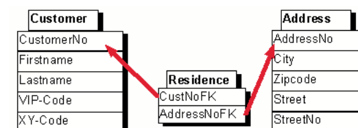
Figure 9: N:M relationship using an associative relation
