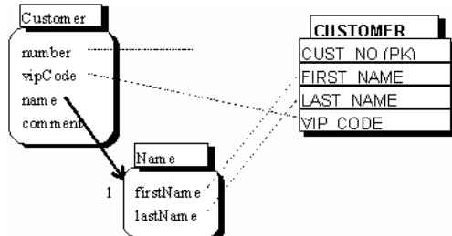
Figure 32: Aggregated Relationship
