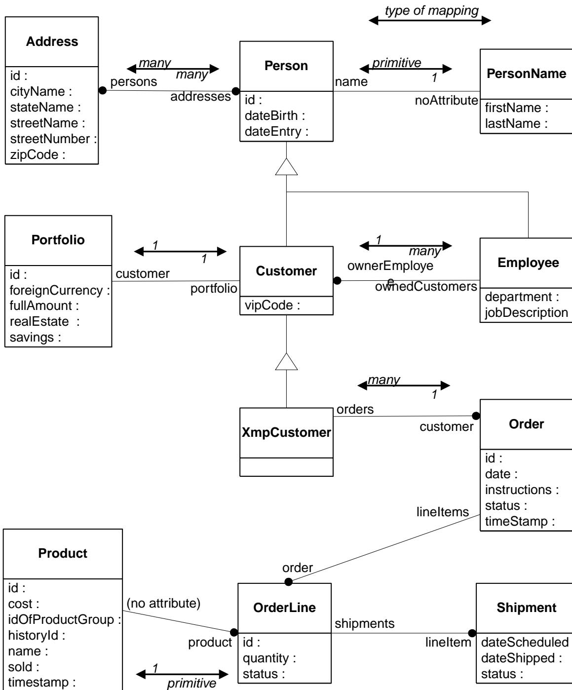
Figure 11: The Customer Base Management class model
