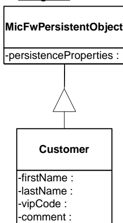
Figure 3: Persistent class derived from MicFwPersistentObject
