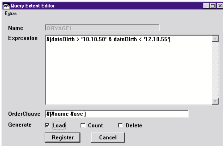
Figure 54: Query editor
