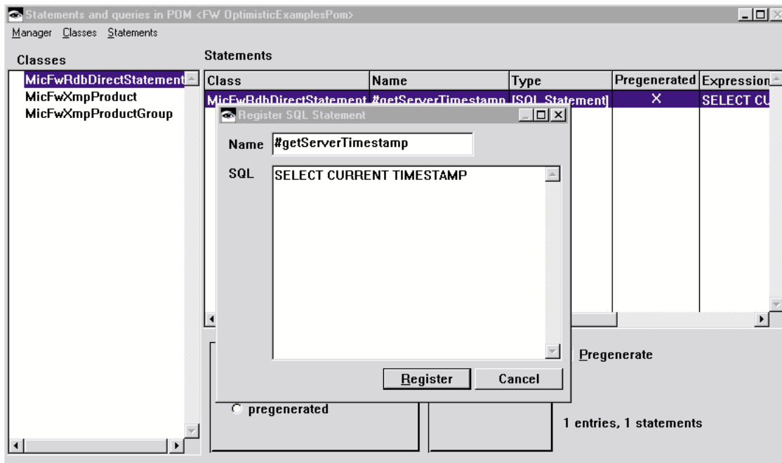
Figure 23: QueryRegistration #getServerTimestamp
