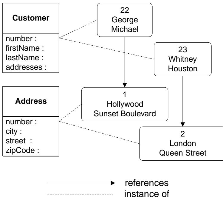
Figure 10: Object Model
