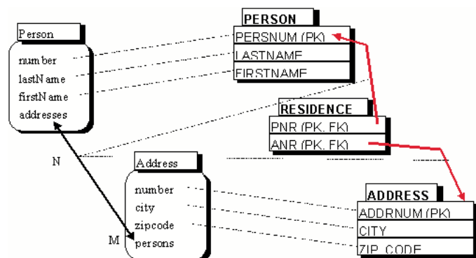
Figure 31: Many-to-Many Relationship
