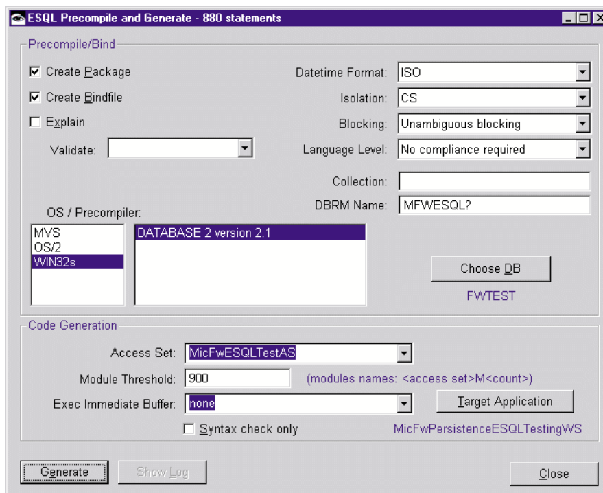
Figure 47: Precompilation Dialog
