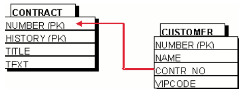
Figure 33: CONTRACT (versioned) and CUSTOMER
