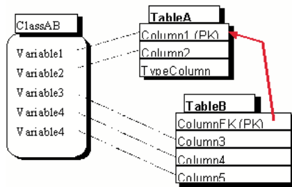
Figure 29: Single class spanning several tables
