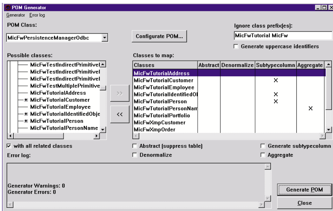
Figure 72: POM generator dialog window
