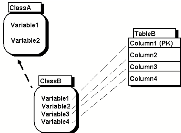
Figure 73: Suppress table
