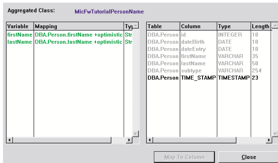
Figure 62: Aggregation editor
