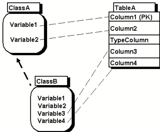
Figure 74: Denormalize table
