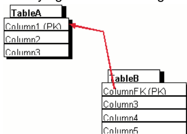
Figure 7: Identifying Relationship
