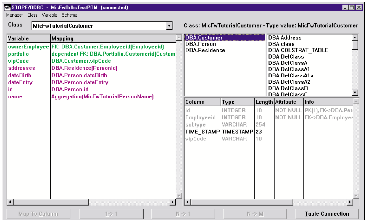
Figure 49: Main view of the STOPF tool
